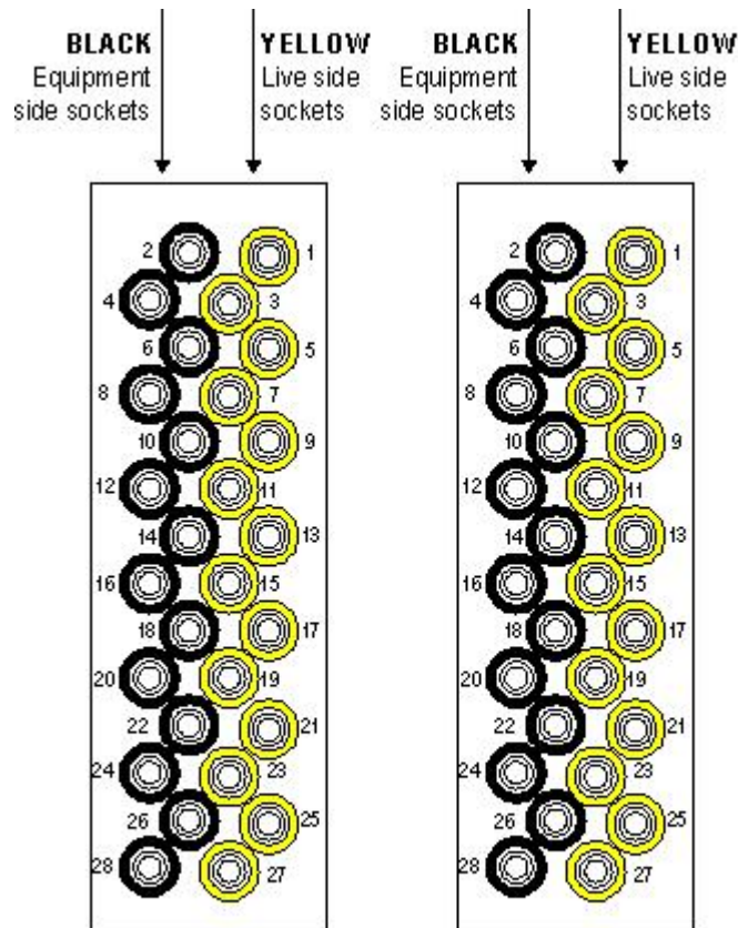
4M422 Test Plug (Front View)
