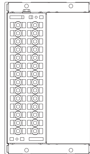
Terminal layout
